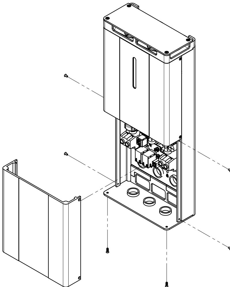
Figure 2: SRX Access Panel Screw Locations
