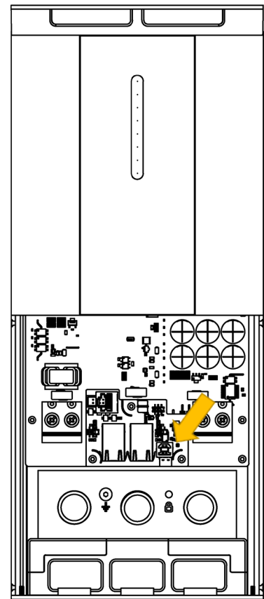
Figure 4: USB-B Programming Port
